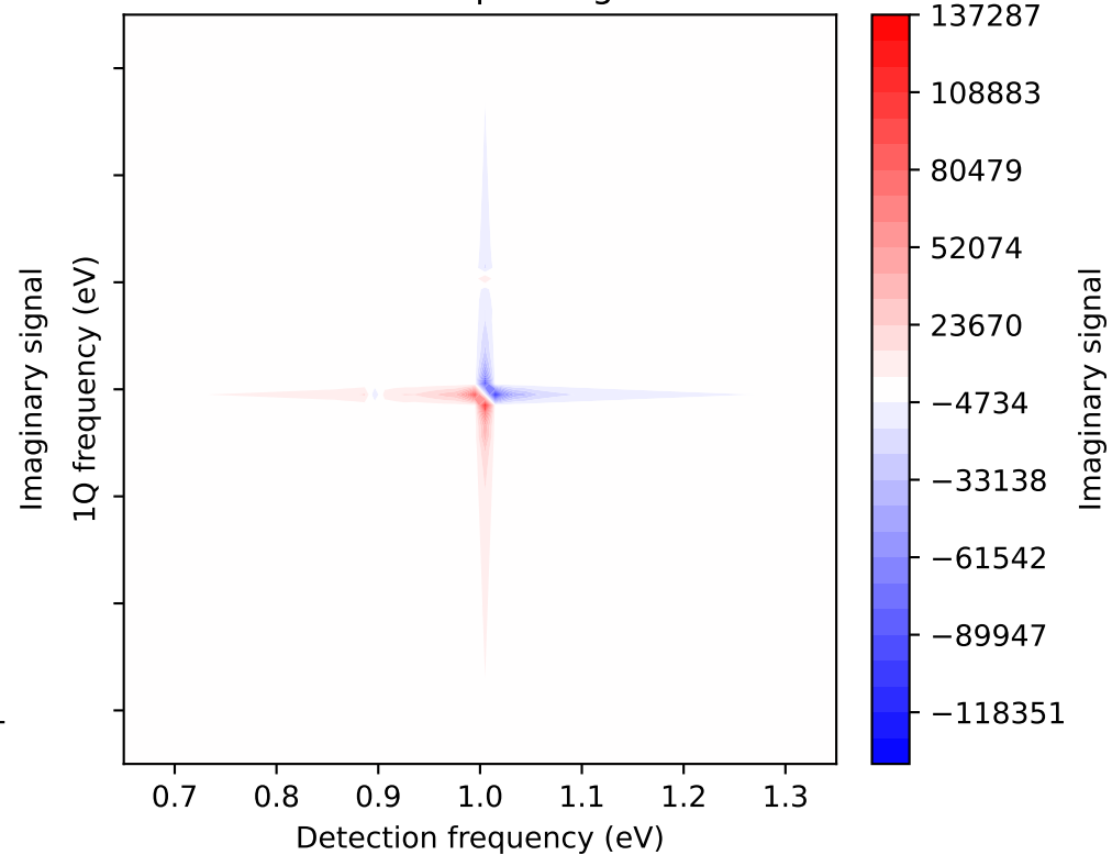
Total rephasing
